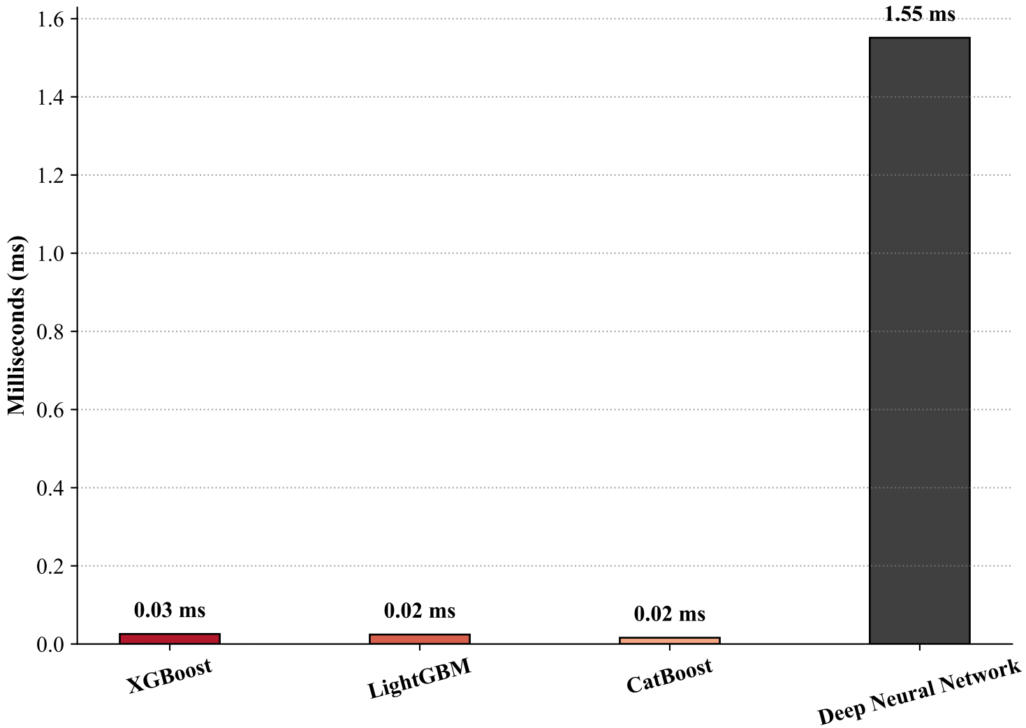
B: Inference Latency (per 1,000 samples)
