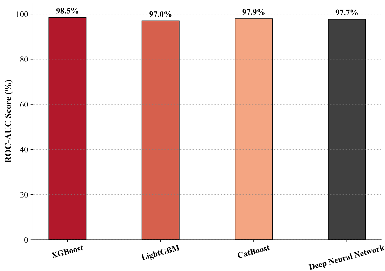
A: Predictive Power (Post-Optimization)
